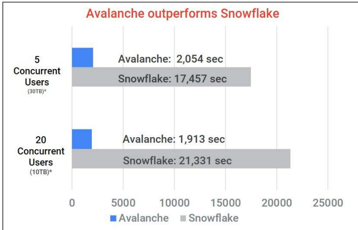
Figure 1: TPC-H benchmark comparisons (Avalanche vs. Snowflake)
