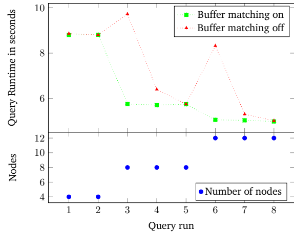
Figure 2: Scaled query performance after adding nodes
