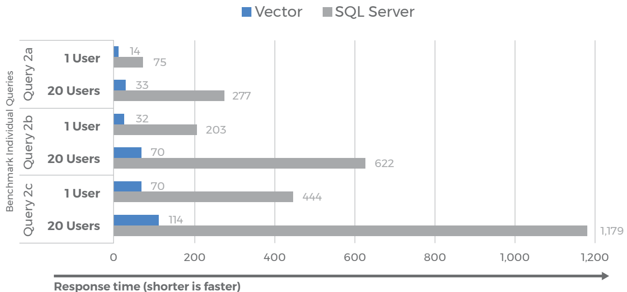
MCG 500GB Aggregation Query Concurrent Execution Median Times
