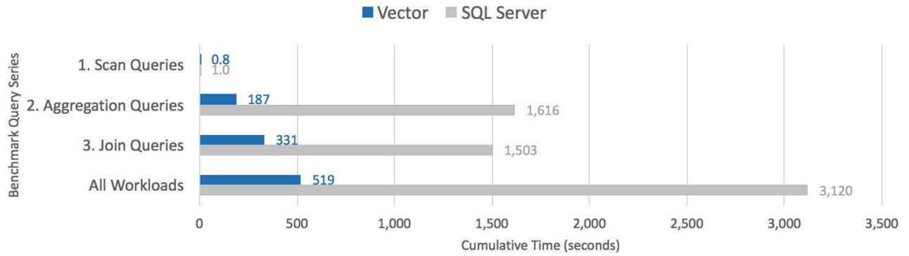
MCG 750GB 20 Concurrent Users Query Set Execution Cumulative Times
