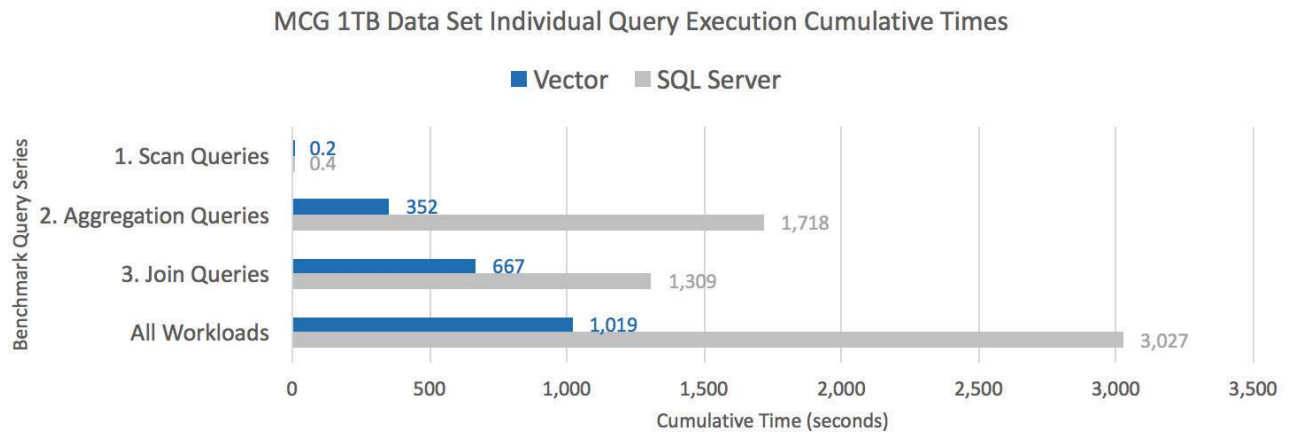
*This graph shows query execution times added together. A shorter bar indicates faster total response times across the workloads.
