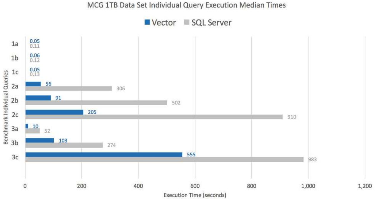
*This graph measures time to execute queries. A shorter bar indicates a faster response time.
