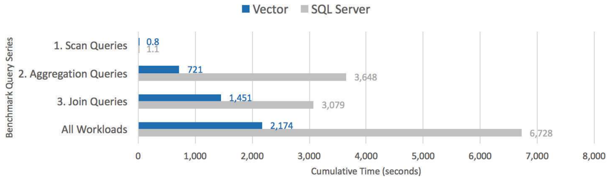
MCG 500GB Data Set Individual Query Execution Cumulative Times
