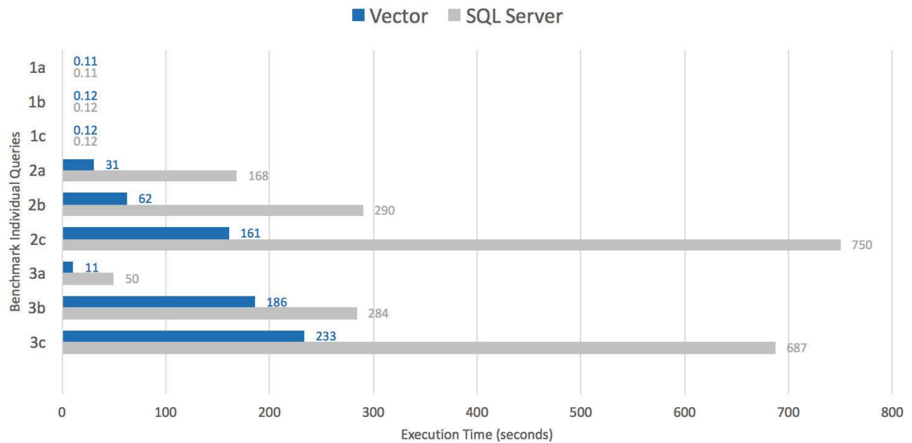
MCG 750GB Data Set Individual Query Execution Median Times
